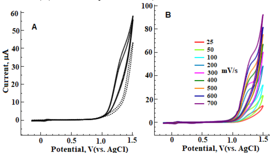
Fig. 1. Cyclic voltammograms for 5.51 mM Metformin at PG electrode in 0.1 M NaOH A) Repeat cycle voltammograms; scan rate, 100 mVs -1 . Dashed line, supporting electrolyte. B) different scan rates.
