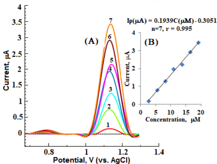
Fig. 5. Square-wave voltammograms for urine sample (A) Metformin not added (dashed line), 1) 2.755 \mu\text{M} 2) 5.51 \mu\text{M} 3) 8.265 \mu\text{M} 4) 11.02 \mu\text{M} 5) 13.775 \mu\text{M} 6) 16.53 \mu\text{M} 7) 19.285 \mu\text{M} (B) the inset depicts the corresponding analytical curve. SW parameters as indicated in Fig. 3.
