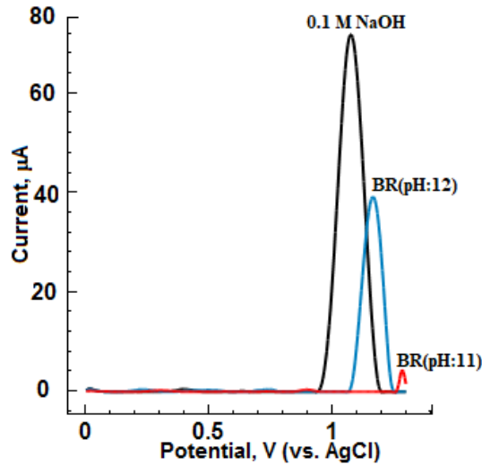
Fig. 3. Square-wave voltammograms for 5.51 mM Metformin in BR (pH:11, 12) and 0.1 M NaOH supporting electrolytes using PG electrode. SW parameters: frequency, 40 Hz; step potential, 8 mV; amplitude, 50 mV.
