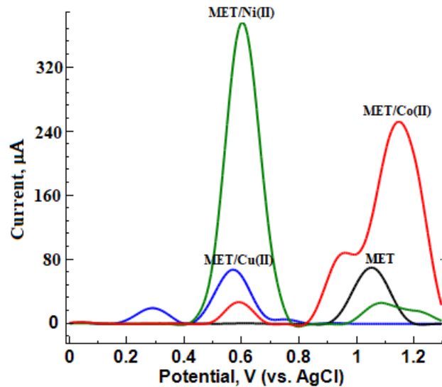
Fig. 6. Square-wave voltammograms for 5.51 mM Metformin mixed with Cu (II), Ni (II) and Co (II) in 0.1 M NaOH using PG electrode
