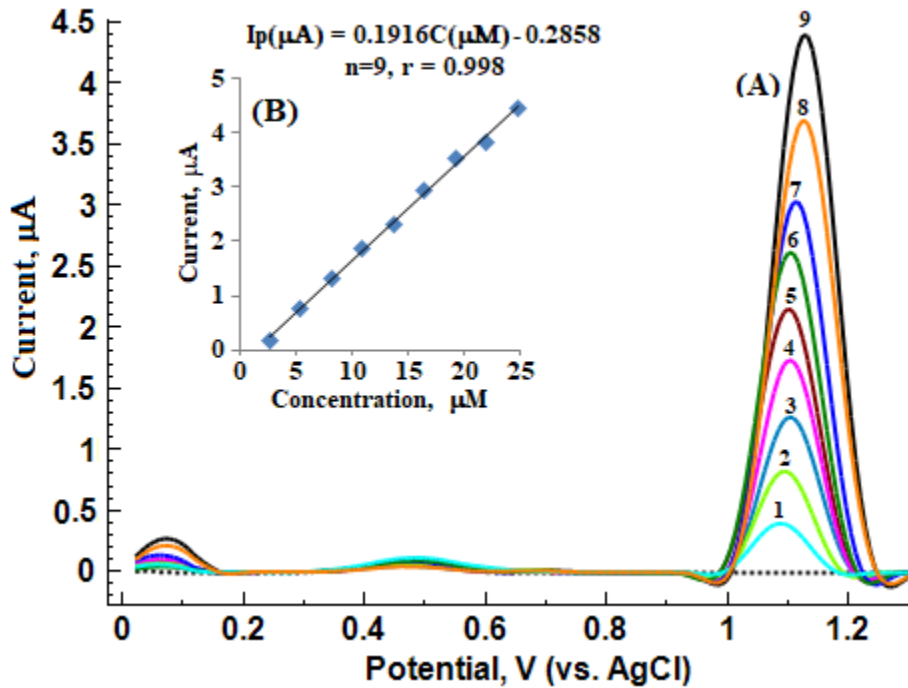
Fig. 4. Square-wave voltammograms for A) Metformin [1] 2.755, 2) 5.51, 3) 8.265, 4) 11.02, 5) 13.775, 6) 16.53, 7) 19.285, 8) 22.04, 9) 24.795 \mu\text{M} ] in 0.1 M NaOH solution using PG electrode. (B): i_p/C_{\text{Metformin}} curve. Dashed line, supporting electrolyte. SW parameters as indicated in Fig. 3.
