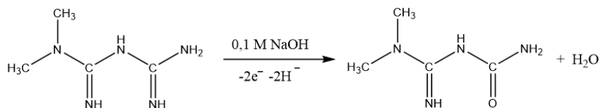
Fig. 2. Possible oxidation mechanism of metformin
