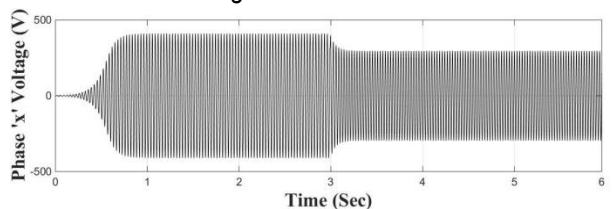
Fig. 16: Voltage of phase 'x' with a load switching time= 3Sec
