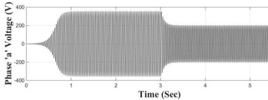
Fig. 9. Voltage of phase 'a' with a load switching time= 3Sec
