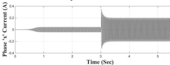
Fig. 12. Current of phase 'x' with a load switching time= 3Sec
