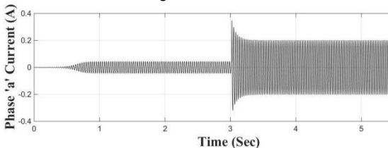
Fig. 11. Current of phase 'a' with a load switching time= 3Sec
