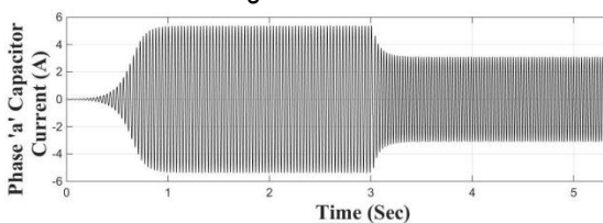
Fig. 13. Capacitor current of phase 'a' with a load switching time= 3Sec
