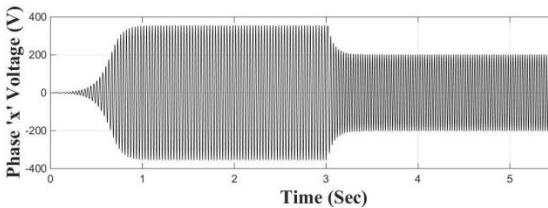
Fig. 10. Voltage of phase 'x' with a load switching time= 3Sec
