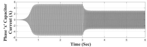
Fig. 14. Capacitor current of phase 'x' with a load switching time= 3Sec Sudden switching of load with series compensation
