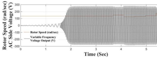
Fig. 17. Varying frequency voltage generation with the change of rotor speed
