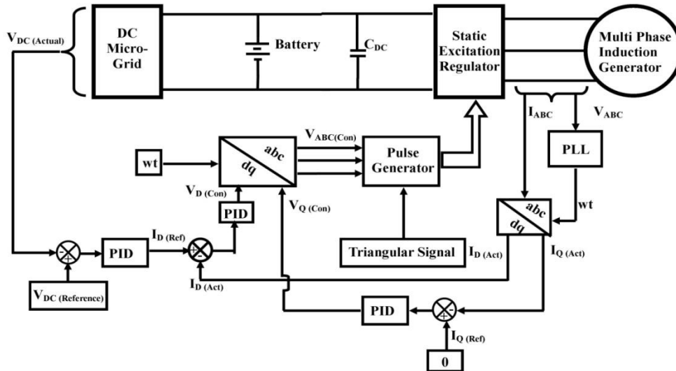
Fig. 5. Control topology for DC side power generation
