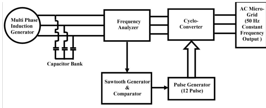
Fig. 4. Control topology for AC side power generation
