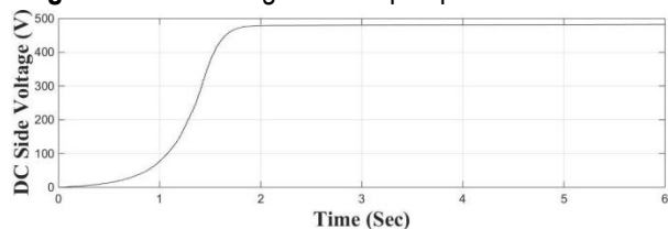
Fig. 8. No load DC side generated voltage from SER
