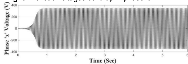
Fig. 7. No load voltages build up in phase 'x'
