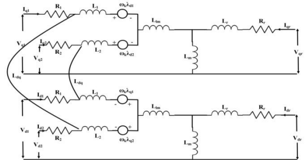
Fig. 3. Equivalent circuit diagram of multi phase induction generator
