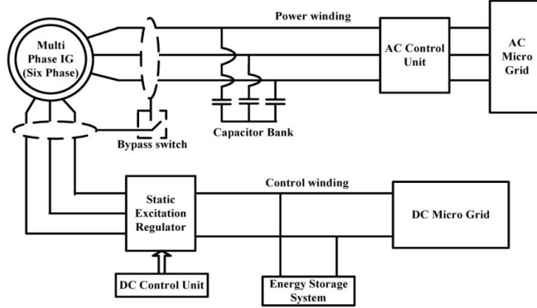
Fig. 1. Structure of proposed standalone AC & DC hybrid micro grid generating system based on multi phase induction generator
