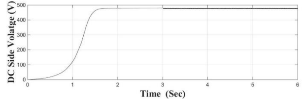
Fig. 19. Voltage of DC side with a load switching time = 3 Sec
