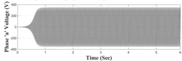
Fig. 6. No load voltages build up in phase 'a'
