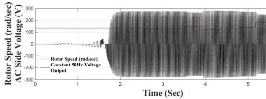
Fig. 18. Constant frequency voltage generation with the varying rotor speed
