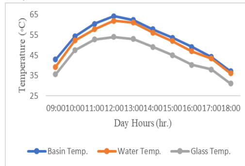
Fig.3. Variation of the basin, water, and inner glass temperature of the conventional solar still
