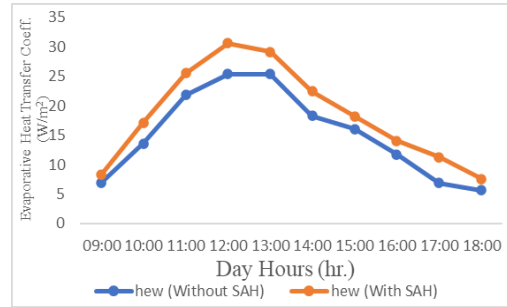
Fig. 7. Evaporative heat transfer for conventional and modified solar still.
