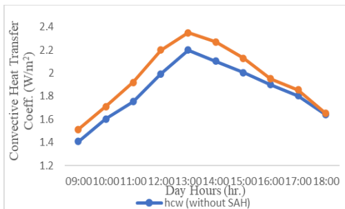
Fig.6. Convective heat transfer for conventional and modified solar still
