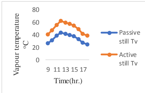
Fig. 5. Vapor Temperature for the modified and conventional Solar Still.
