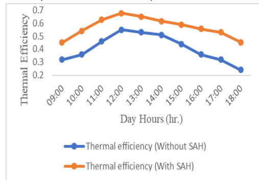
Fig. 8. Hourly variation of thermal efficiencies of the conventional and modified solar stills Conventional solar distillation Thermal Efficiency = (Yield Output × Latent heat of Vaporization) / Incident energy on solar still × 100%
