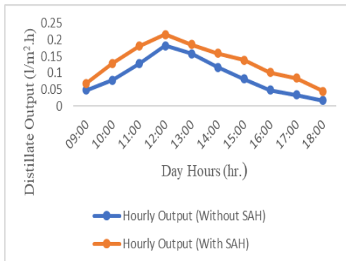
Fig.9. Freshwater yield of the conventional and modified solar still
