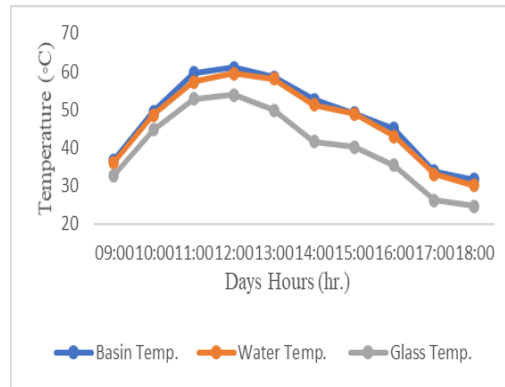
Fig.3. Variation of the basin, water, and inner glass temperature of the conventional solar still
