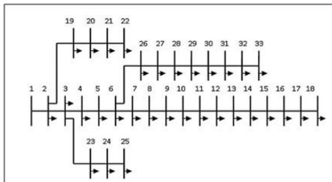
Fig. 3. IEEE 33 Bus distribution system
