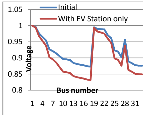
Fig. 5. Voltage graph with EV Station only In Above Fig. 5. Represents the voltage profile of the all the two cases that is initial and with EV only.
