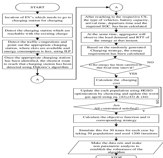
Fig. 5. Flowchart of the work process
