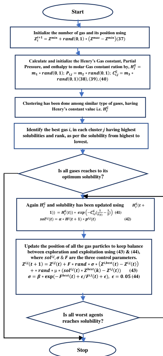
Fig. 4. Flowchart for HGSO
