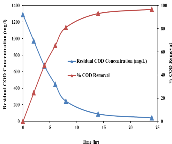
Fig. 1. Carbon oxidation profile in batch reactor [initial COD = 1289 mg/L]
