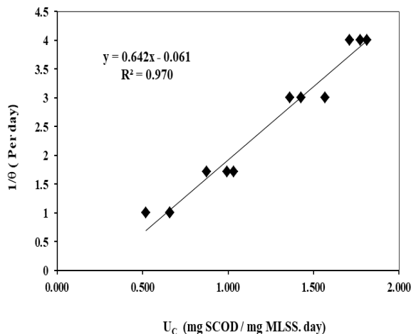
Fig. 9. Graphical plot for microbial growth kinetics for carbon oxidation.
