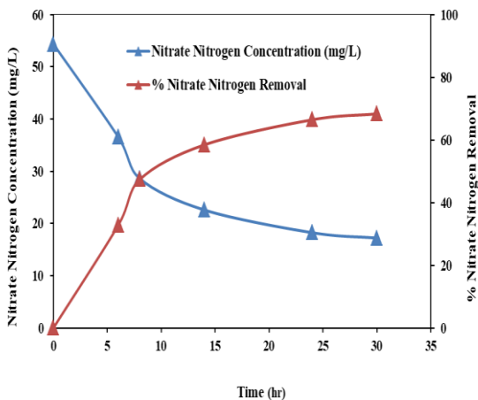
Fig. 5. Nitrate nitrogen removal profile in batch reactor [initial \text{NO}_3^- -N = 54.36 mg/L]
