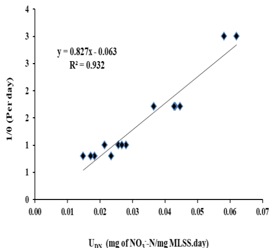
Fig. 13. Graphical plot for microbial growth kinetics for denitrification.
