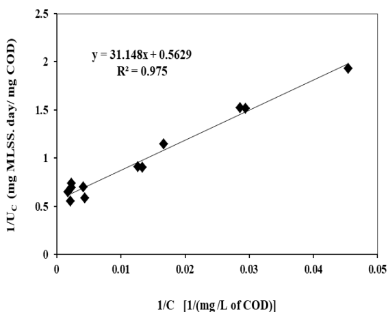
Fig. 8. Graphical plot for substrate utilization kinetics for Carbon oxidation
