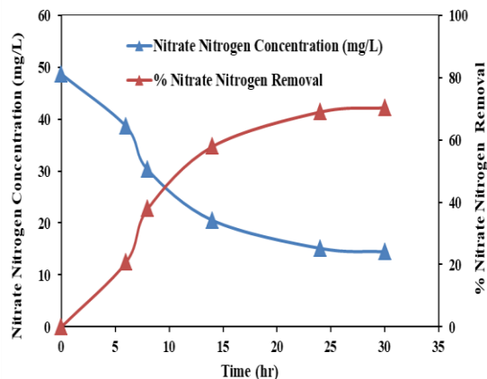
Fig. 6. Nitrate nitrogen removal profile in batch reactor [initial \text{NO}_3^- -N = 48.67 mg/L]
