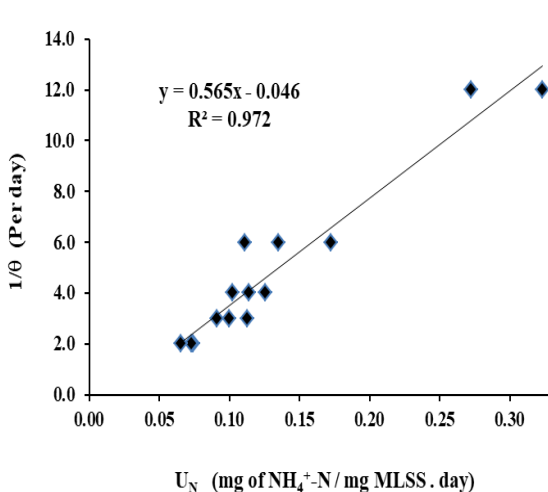
Fig. 11. Graphical plot for microbial growth kinetics for nitrification.
