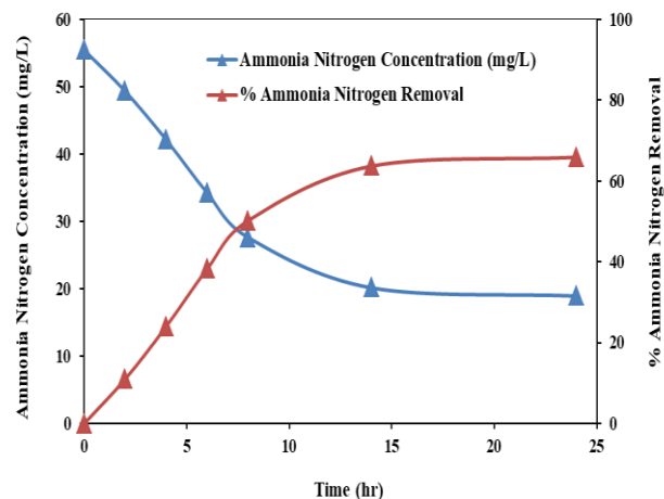
Fig. 3. Ammonia nitrogen removal profile in batch reactor [initial \text{NH}_4^+\text{-N} = 55.4 mg/L]
