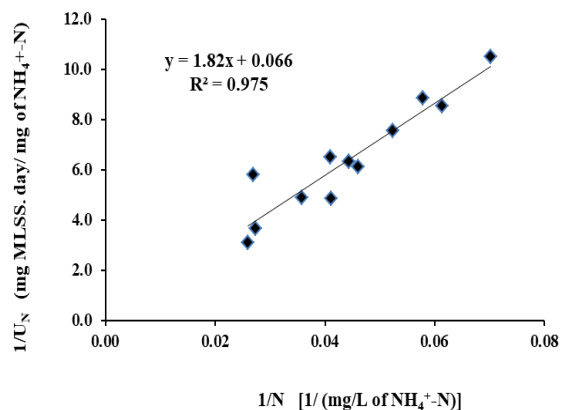
Fig. 10. Graphical plot for substrate utilization kinetics for nitrification.
