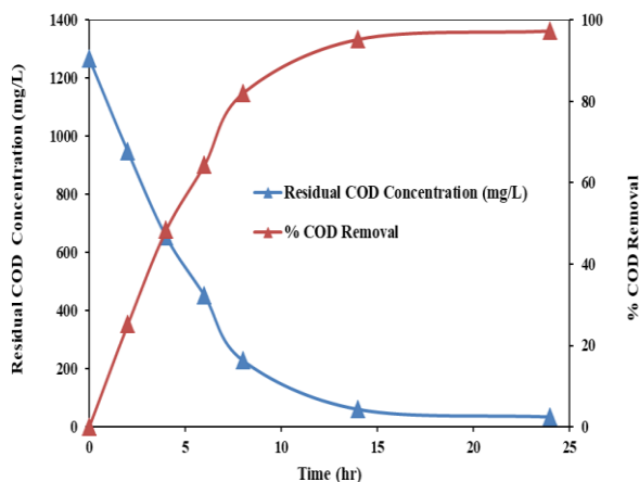
Fig. 1. Carbon oxidation profile in batch reactor [initial COD = 1289 mg/L]
