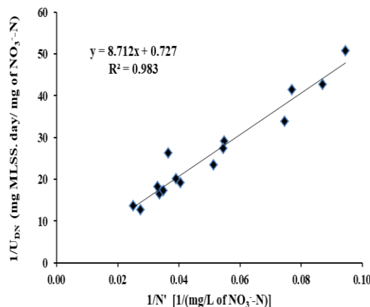
Fig. 12. Graphical plot for substrate utilization kinetics for denitrification
