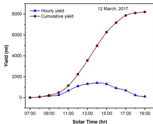
Fig.6. Variation (hourly) of yield & cumulative yield versus solar time
