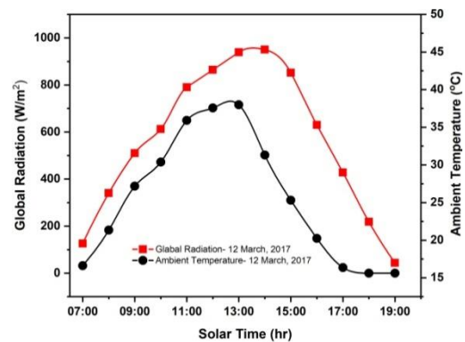
Fig.4. Variation (hourly) of global radiation & ambient temperature versus solar time
