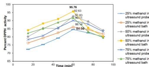
Fig.10. Percentage DPPH radical scavenging activity [1:25 ratio]
