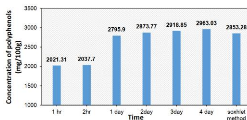
Fig.7. Extraction of polyphenols conventional and Soxhlet method [Solvent: 50% methanol; 1:25 ratio]
