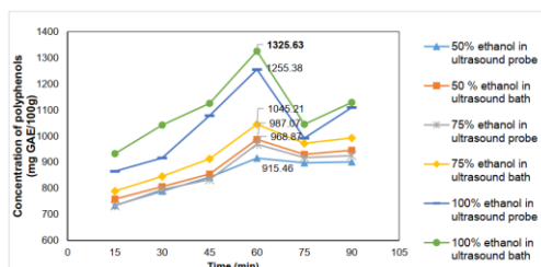
Fig.5. Polyphenolic yield using ethanol as solvent [1:25 ratio]
