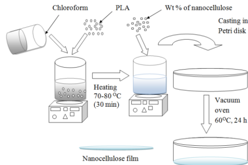
Fig. 1. Preparation of bagasse nanocellulose film
