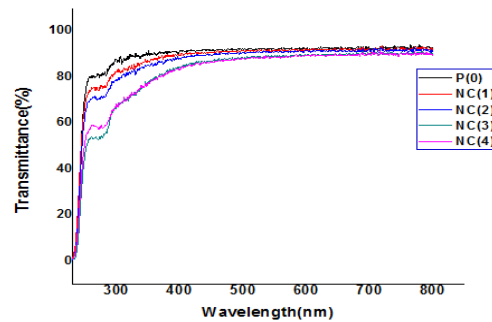
Fig. 3. Transmittance v/s wavelength graph of nanocellulose films
