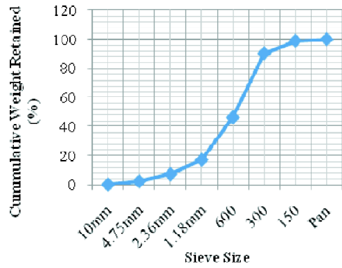
Fig. 1. Grading of fine aggregate.
