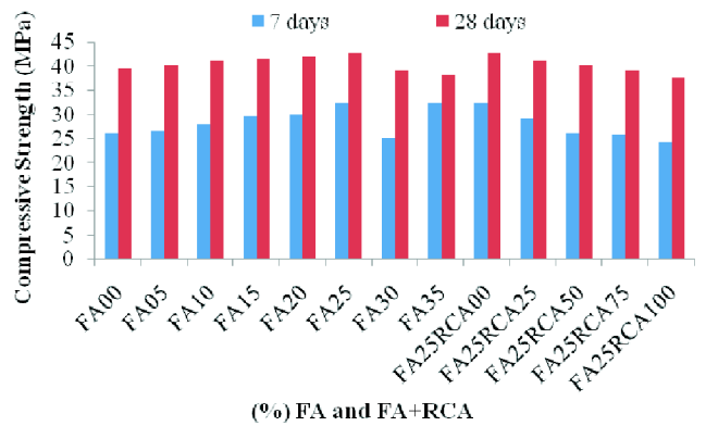
Fig. 8. Compressive strength of SCC mixes.
