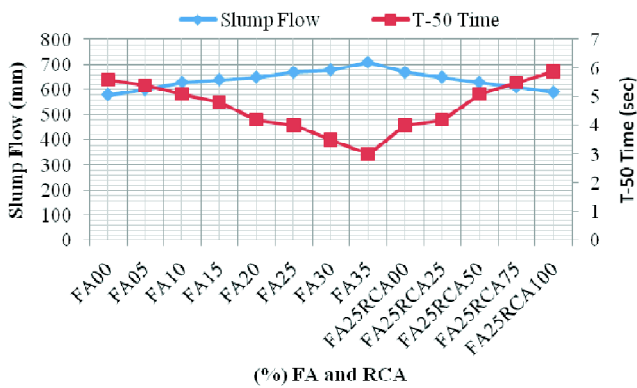
Fig. 5. Slump flow vs T-50 time.
