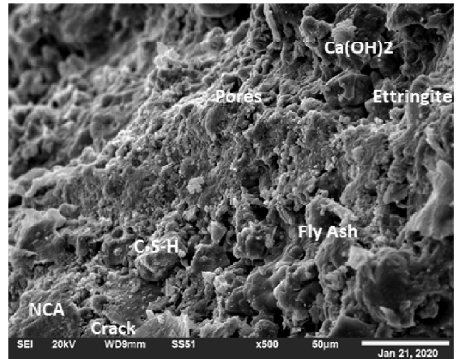
Fig. 11. SEM micrograph of FA25 at 28 days.
