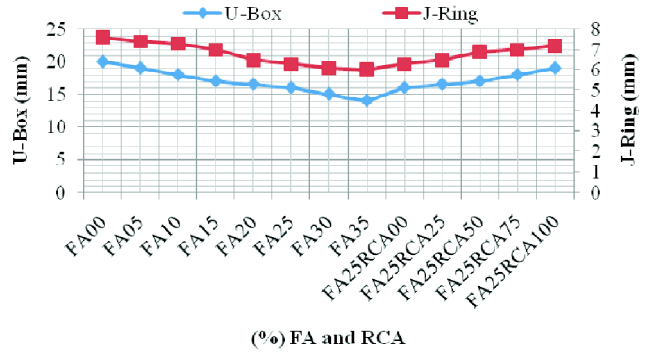
Fig. 7. U-Box vs J-ring.
