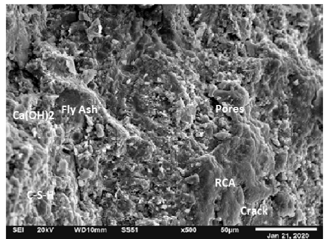
Fig. 12. SEM micrograph of FA25RCA25 at 28 days.
