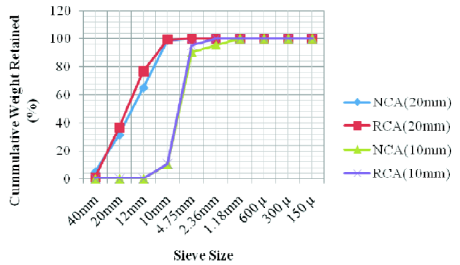
Fig. 2. Grading of NCA and RCA (10 and 20 mm).
