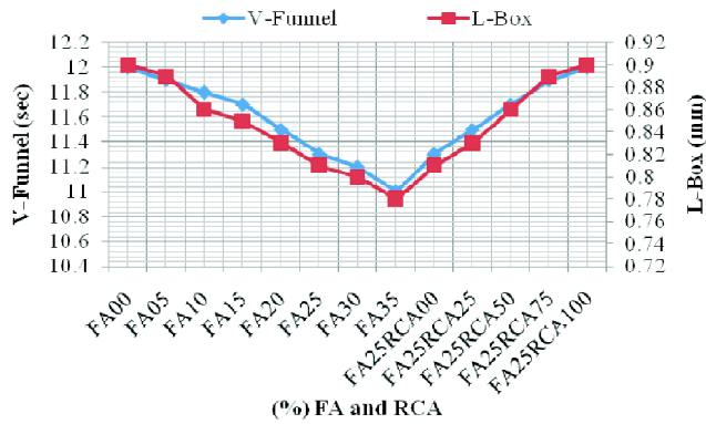
Fig. 6. V-Funnel vs L-box
