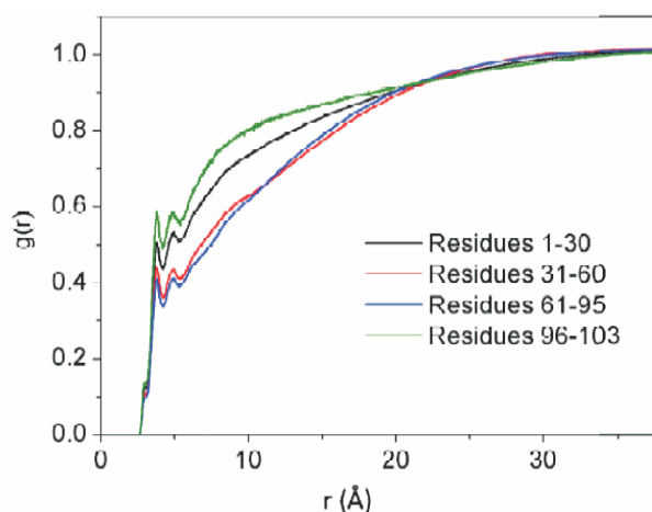
Fig. 4. The pair radial distribution function, g(r) , between the backbone heavy atoms of each domain of AS(1-103) and the oxygen atoms of the water molecules.
