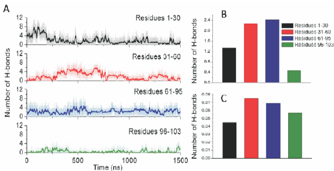
Fig. 3. (A) The time evolution of the number of backbone hydrogen bonds formed in different domains of AS(1-103) along a simulation trajectory (light colours) and the corresponding 500-point running averages are shown in dark colours (B) the time-averaged hydrogen bonds formed by different domains over last 1250 ns of the simulation trajectory. (C) The time-averaged hydrogen bonds divided by the number of residues of the corresponding domain.
