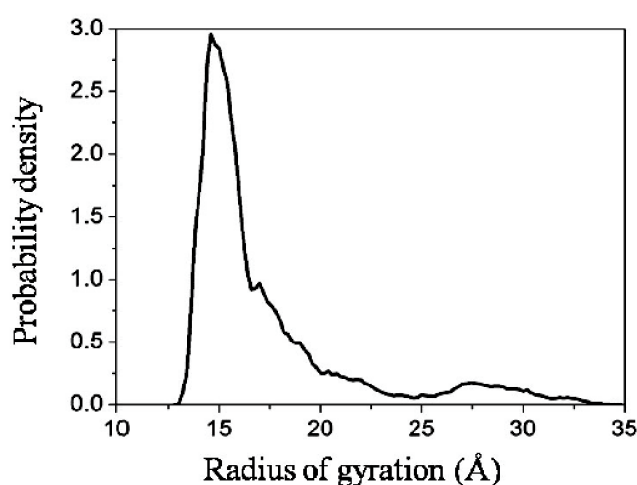
Fig. 6. Probability distribution of the radius of gyration ( R_g ).
