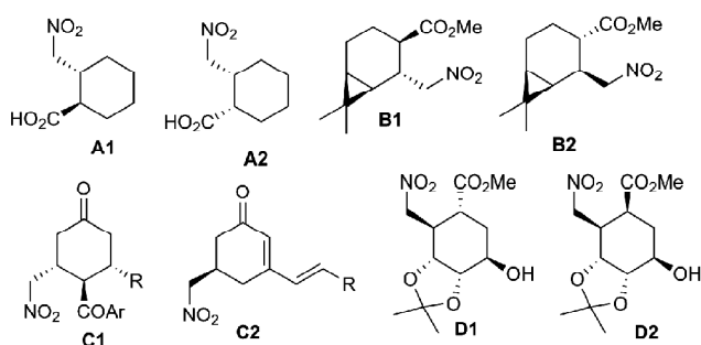
Fig. 1. Selected cyclohexanes 7 functionalized with \text{CH}_2\text{NO}_2 group.
